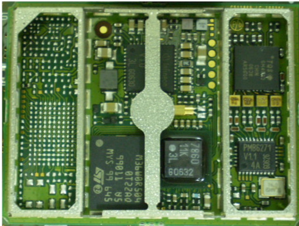
Photograph No.22 GE863-Quad module internal view
